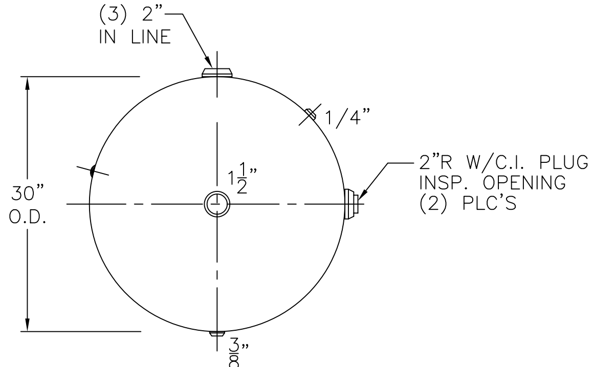
VIEW W/OUT SUPT.
